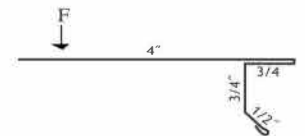
⑥⑩ Drip Edge 10'2" TL6.5F60xx
