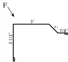
⑱ Residential Rake 10'2" TLRR18xx
