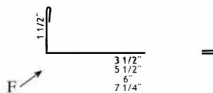
⑩ Post Trim 10'2" TLPT10xx
