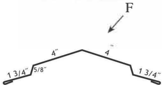
① 13" Univ. Ridge 10'6" TLURC1xx
