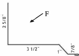
⑧ Univ. Sidewall 10'2" TLUS8xx
